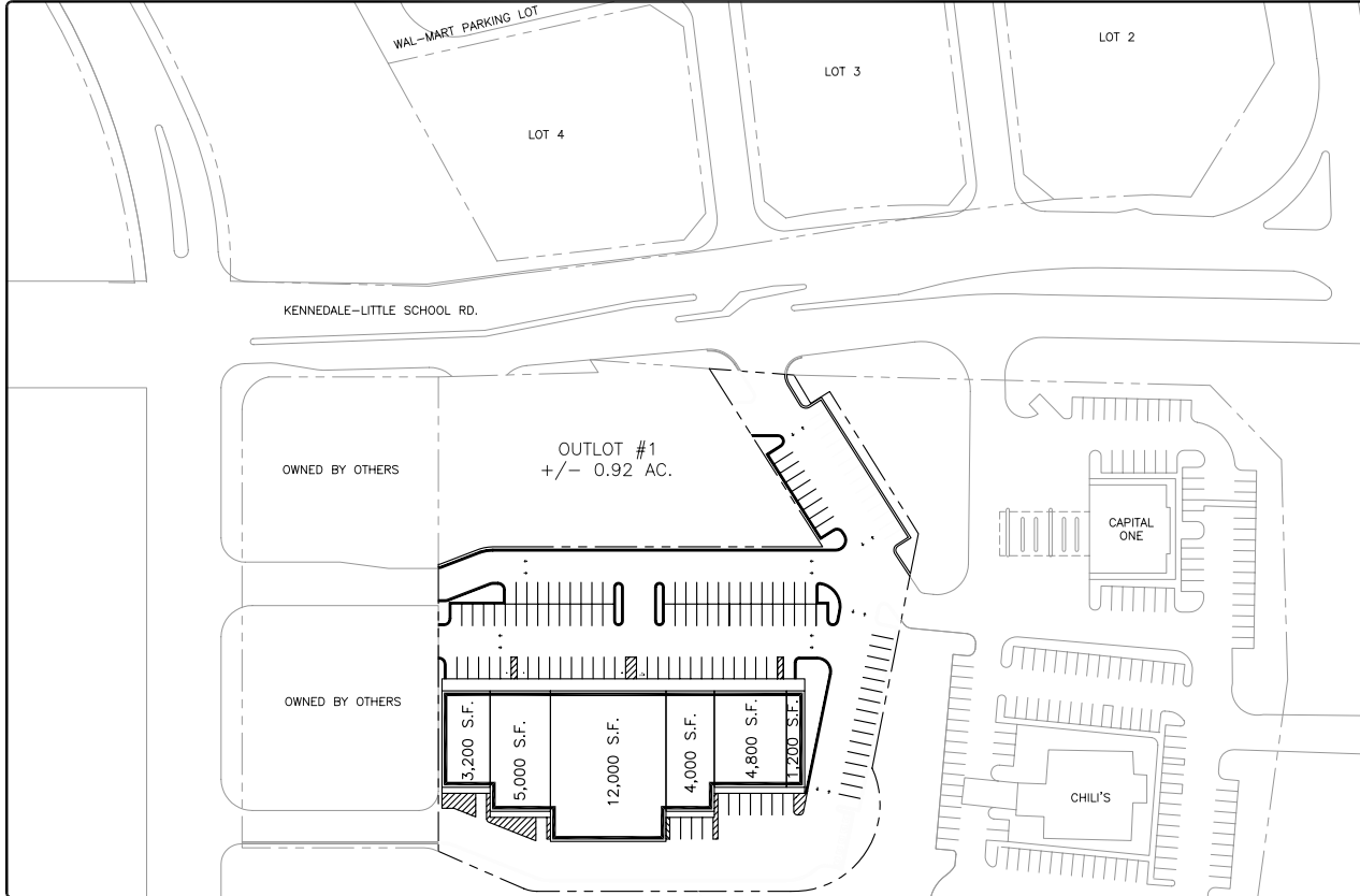
SITE DEVELOPMENT PLAN
