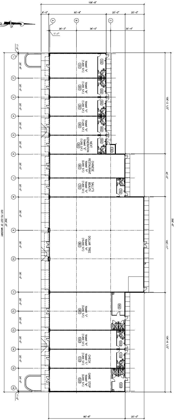
1 FLOOR PLAN 1/16" = 1'-0"
